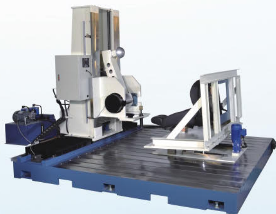
HT-2120 汽車座椅頭枕測試試驗台 Computer Servo Control Headrest Impact Tester
