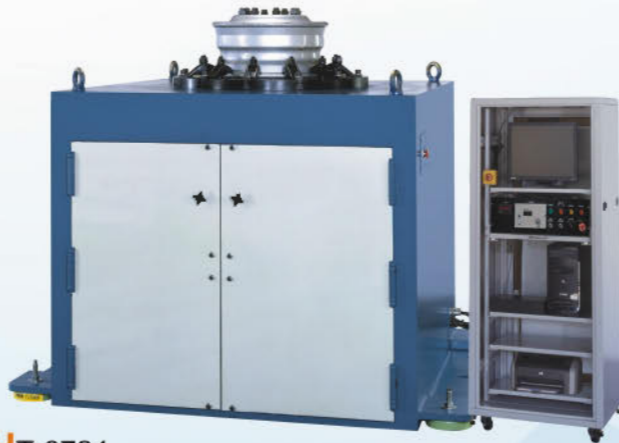
HT-2724 輪圈彎曲力矩耐久試驗機 Cornering Fatigue Testing Machine Capacity : 5000, 20000, 35000 N-m
