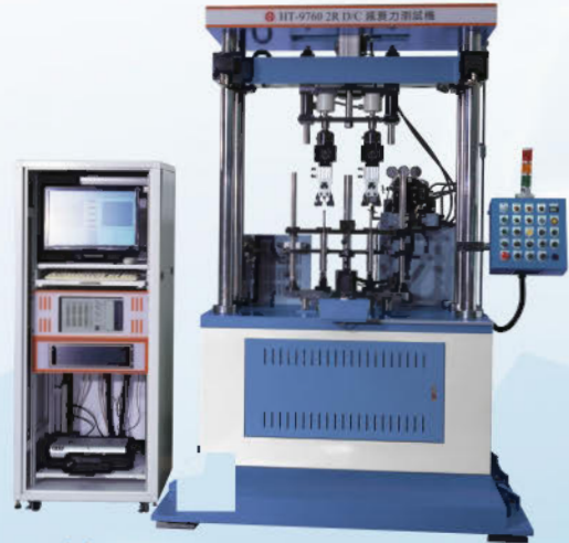
HT-9760-2R 衰減力試驗機 (雙軸式) Damping Tester (Two Stations)
